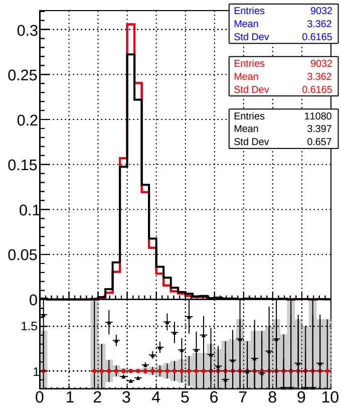
Legend: DQM_mkFit_time (blue line with squares) DQM_mkFit_time_b1 (red line with circles) DQM_BDT_mkFit_time (black line with crosses)
