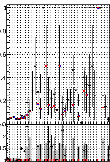
Fake rate vs. —•— DOM mkFit time —•— DOM B0Fit time b1 —•— DOM B0Fit mkFit time
