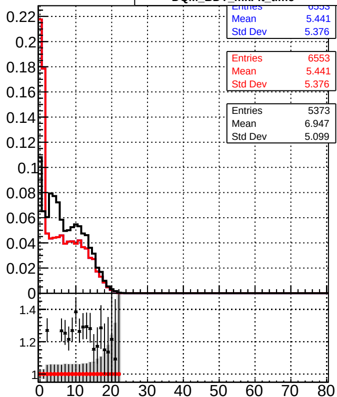
Legend for bottom row: DQM_mkFit_time (Blue line with squares) DQM_mkFit_time_b1 (Red line with circles) DQM_BDT_mkFit_time (Black line with crosses)
