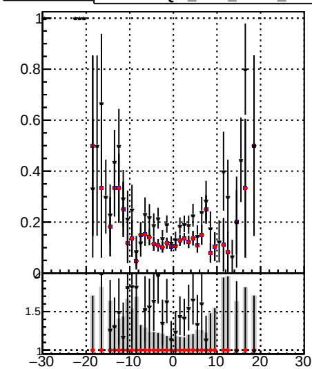
—●— DQM_mkFit_time —●— DQM_mkFit_time_b1 —●— DQM_BDT_mkFit_time
