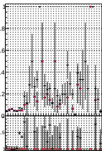
Fake rate vs. DOM mkFit time DOM B0Fit time DOM B0Fit time
