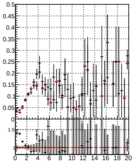
Fake rate vs. DOM mkFit time DOM B0Fit time DOM B0Fit time
