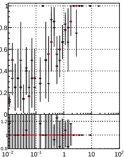
—•— DOM_mkFit_time —•— DOM_mkFit_time_b1 —•— DOM_BDT_mkFit_time
