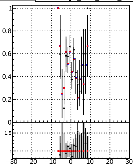
—•— DOM_mkFit_time —•— DOM_mkFit_time_b1 —•— DOM_BDT_mkFit_time
