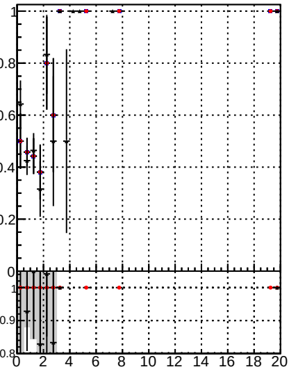
Fake rate vs. BQM mkFit time BQM BDT mkFit time b1 BQM BDT mkFit time
