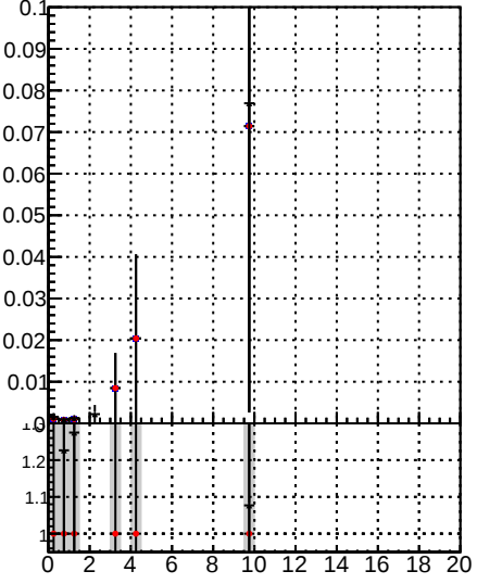
Fake rate vs. — DOM mkFit time — DOM BDT time b1 — DOM BDT mkFit time
