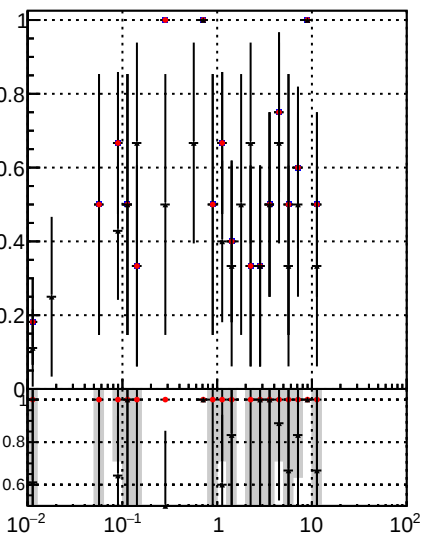
Fake rate vs v —●— DQM mkFit time —●— DQM mkFit time b1 —●— DQM_BDT_mkFit_time
