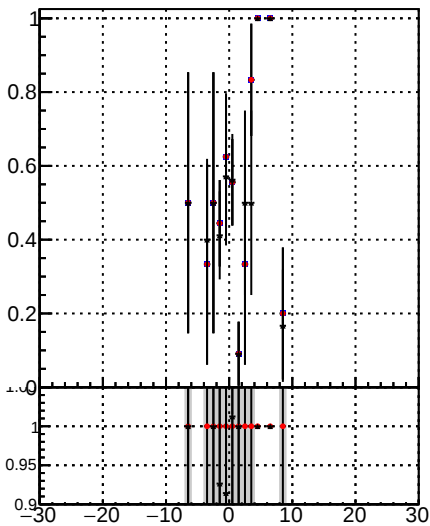
Fake rate vs v —●— DQM mkFit time —●— DQM mkFit time b1 —●— DQM_BDT_mkFit_time
