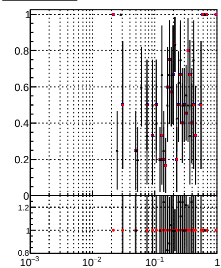
Fake rate vs \sqrt{s} Legend: DOM_mkFit_time DOM_mkFit_time_b1 DOM_BDT_mkFit_time
