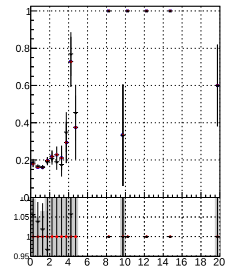
Fake rate vs. DOM mkFit time DOM BDT mkFit time b1 DOM BDT mkFit time
