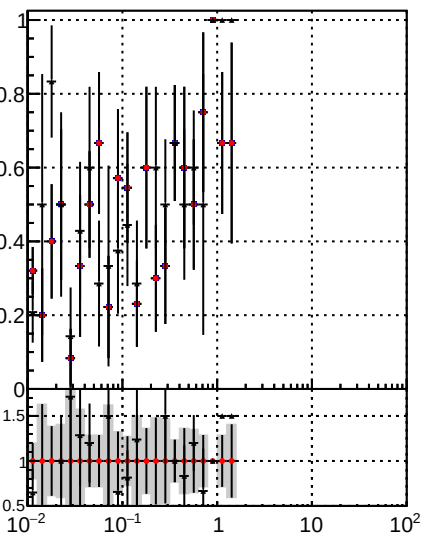
Fake rate vs v DOM_mkFit_time DOM_mkFit_time_b1 DOM_BDT_mkFit_time
