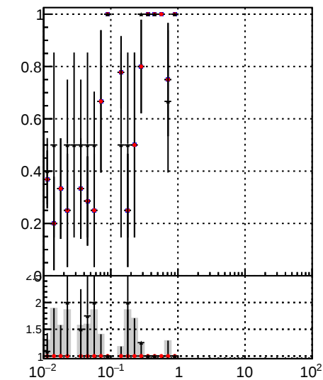
Fake rate vs v Legend: DOM_mkFit_time (gray line) DOM_mkFit_time_b1 (red line) DOM_BDT_mkFit_time (black line)
