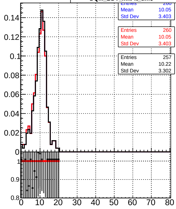
Legend: DQM_mkFit_time (blue line with square markers) DQM_mkFit_time_b1 (red line with circular markers) DQM_BDT_mkFit_time (black line with square markers)
