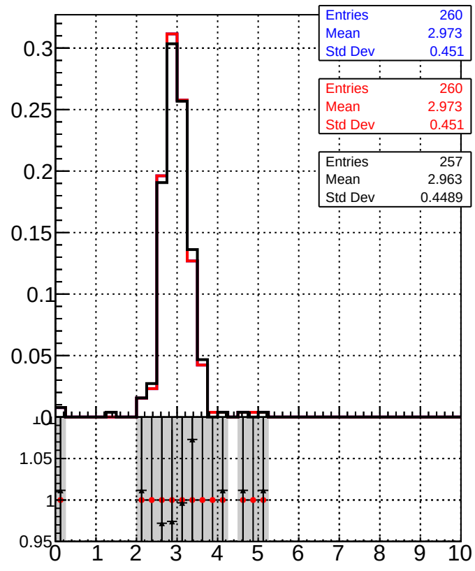
Legend: DQM_mkFit_time (blue line with square markers) DQM_mkFit_time_b1 (red line with circular markers) DQM_BDT_mkFit_time (black line with square markers)
