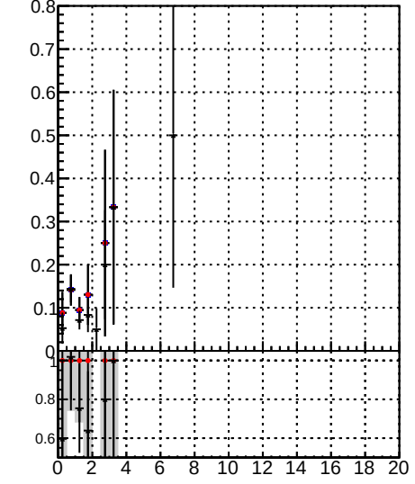
Fake rate vs. \chi^2 for different fit times and b1 values
