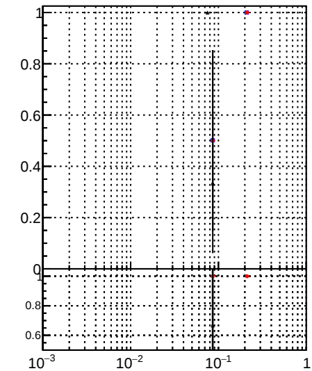
Fake rate vs \sqrt{s} DOM_mkFit_time DOM_mkFit_time_b1 DOM_BDT_mkFit_time
