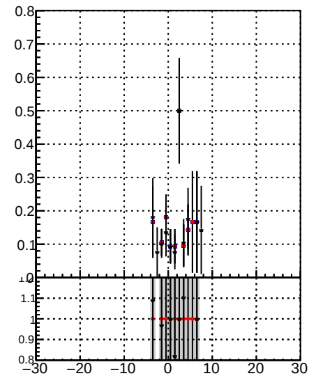
Fake rate vs d —•— DOM mkFit time —•— DOM BDT mkFit time b1 —•— DOM BDT mkFit time
