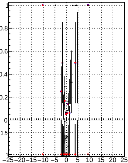
Fake rate vs d —•— DOM mkFit time —•— DOM mkFit time b1 —•— DOM BDT mkFit time
