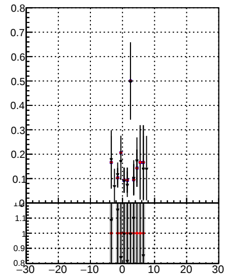
Fake rate vs d — DOM mkFit time — DOM BDT mkFit time — DOM BDT mkFit time b1
