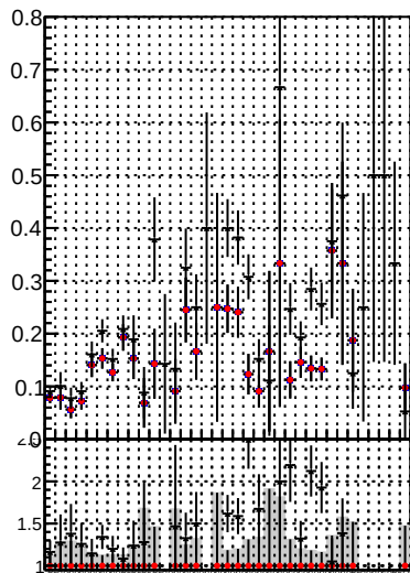
Fake rate vs. — BQM mkFit time — BQM B0F mkFit time — BQM B0F mkFit time b1
