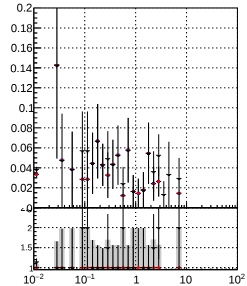
Legend: —●— DQM_mkFit_time —●— DQM_mkFit_time_b1 —●— DQM_BDT_mkFit_time
