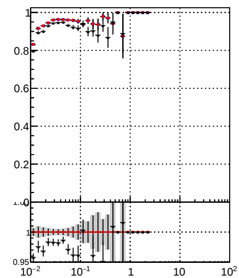
Legend: —●— DQM_mkFit_time —●— DQM_mkFit_time_b1 —●— DQM_BDT_mkFit_time
