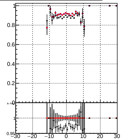
Legend: —●— DQM_mkFit_time —●— DQM_mkFit_time_b1 —●— DQM_BDT_mkFit_time
