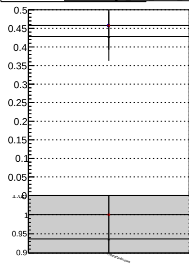
Fake rate vs. DOM mkFit time DOM BDT mkFit time b1 DOM BDT mkFit time
