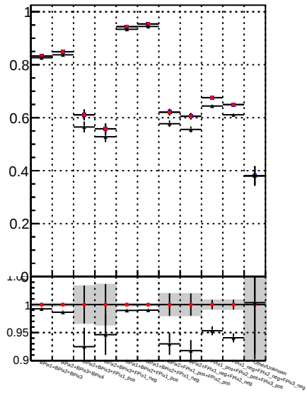
Fake rate vs. — DOM mkFit time — DOM B0Fit time b1
