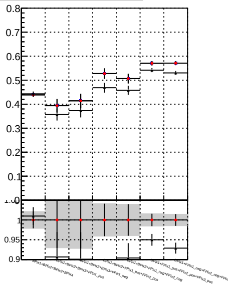
Fake rate vs. — DOM mkFit time — DOM BDT mkFit time
