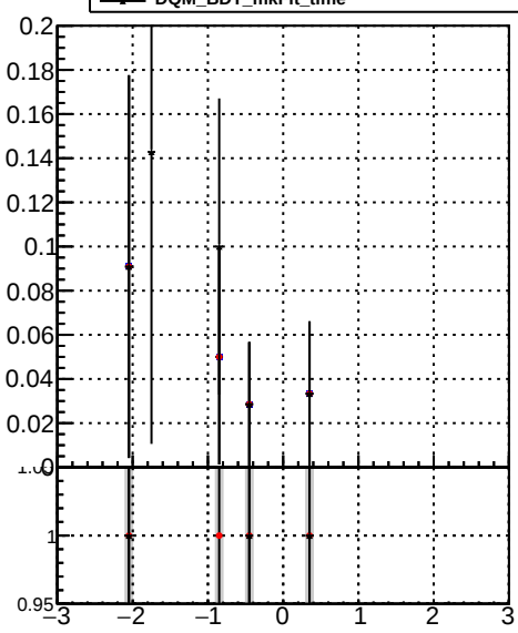
Legend: —•— DQM\_mkFit\_time —•— DQM\_mkFit\_time\_b1 —•— DQM\_BDT\_mkFit\_time
