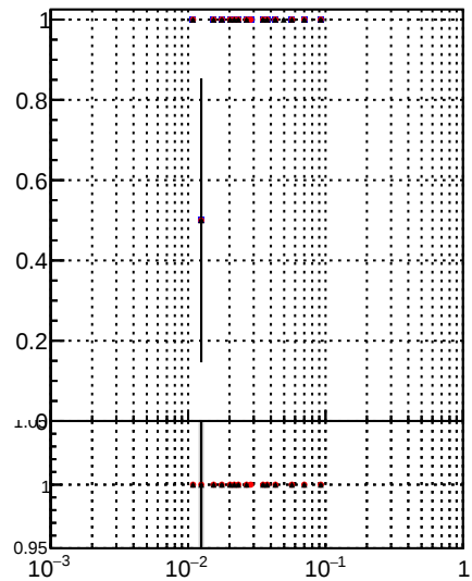
Fake rate vs \epsilon Legend: DQM_mkFit_time (black line) DQM_mkFit_time_b1 (red line) DQM_BDT_mkFit_time (black line)
