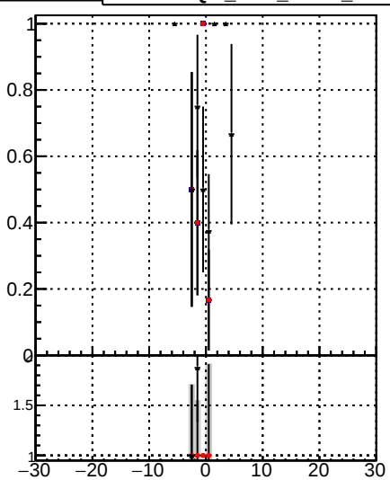
Fake rate vs v —•— DQM_mkFit_time —•— DQM_mkFit_time_b1 —•— DQM_BDT_mkFit_time
