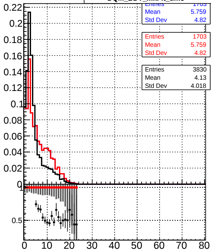
— DQM_mkFit_time — DQM_mkFit_time_b1 — DQM_BDT_mkFit_time
