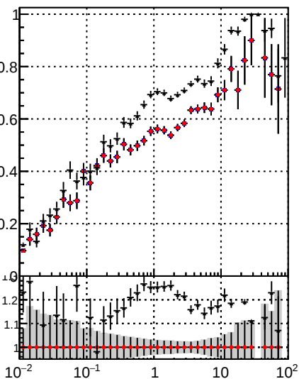
— DQM_mkFit_time — DQM_mkFit_time_b1 — DQM_BDT_mkFit_time
