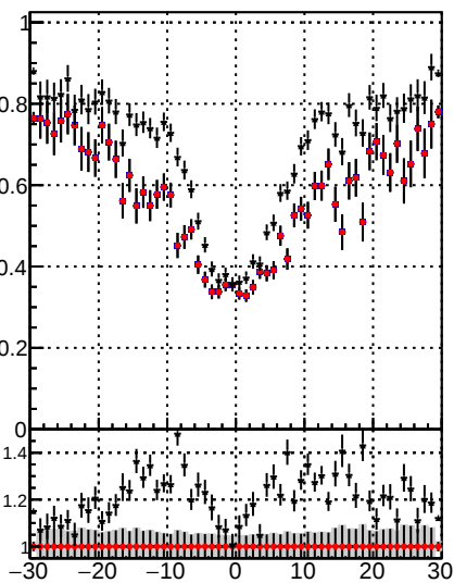
Fake rate vs d —●— DOM mkFit time —●— DOM BDT mkFit time
