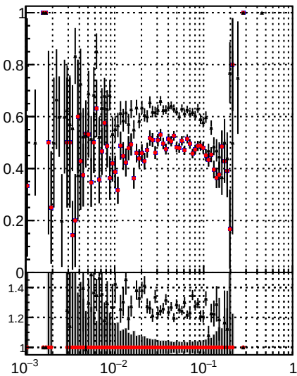
Fake rate vs \mu Legend: DQM mkFit time (black circles) DQM mkFit time b1 (red circles) DQM BDT_mkFit_time (black crosses)
