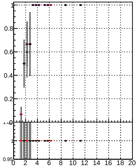
Fake rate vs. DOM mkFit time DOM BDT mkFit time b1
