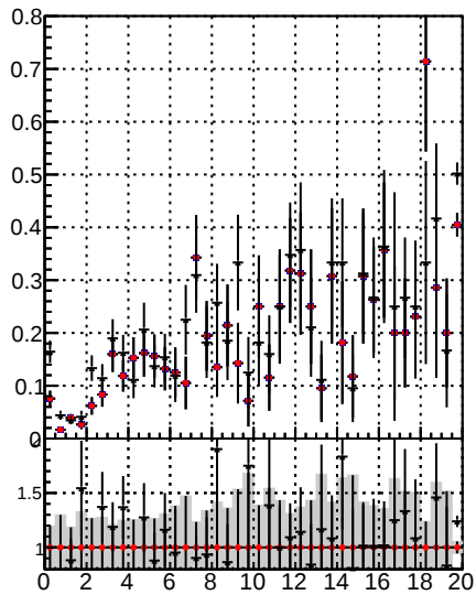
Fake rate vs. —•— DOM mkFit time —•— DOM B0F mkFit time —•— DOM B0F mkFit time b1
