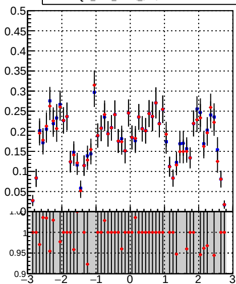
—■— DQM_mkFit_time —●— DQM_BDT_mkFit_time
