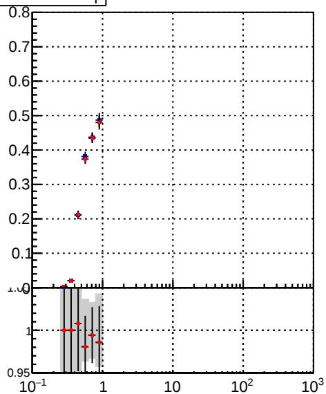
—■— DQM_mkFit_time —●— DQM_BDT_mkFit_time
