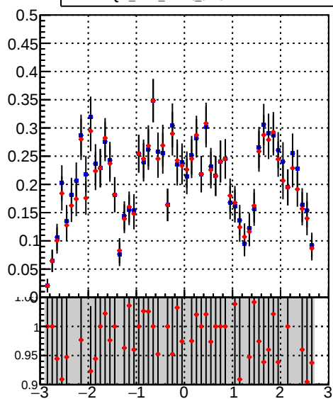
— DQM_mkFit_time — DQM_BDT_mkFit_time
