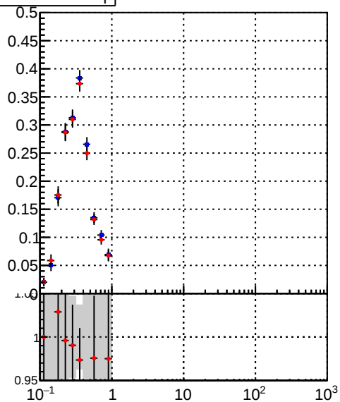
— DQM_mkFit_time — DQM_BDT_mkFit_time
