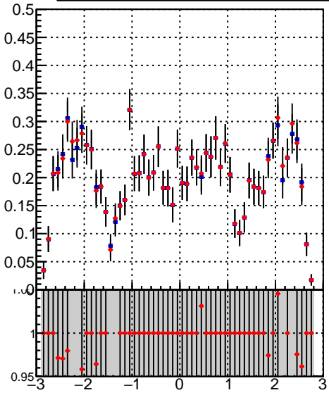
— DQM_mkFit_time — DQM_BDT_mkFit_time
