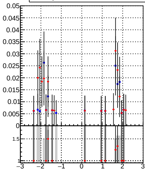
— DQM_mkFit_time — DQM_BDT_mkFit_time
