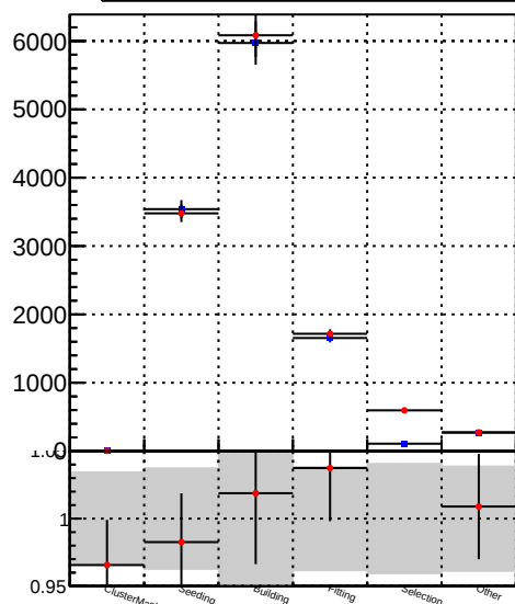
Average —●— DQM_BDT_mkFit_time
