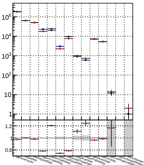
Number of iterations: 1000000 Legend: DQM_mkFit_time DQM_BDT_mkFit_time
