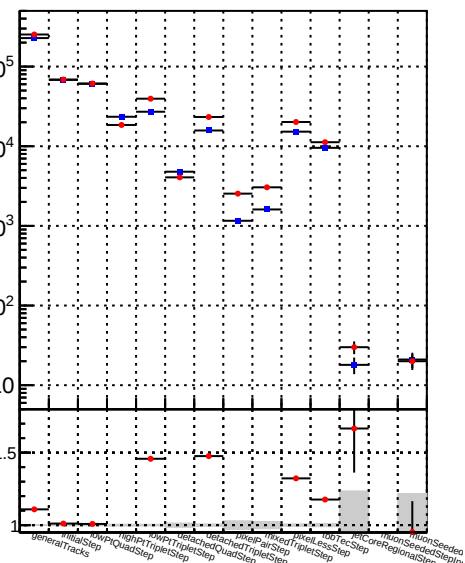
Number of iterations: 1000000 Legend: DQM_mkFit_time DQM_BDT_mkFit_time
