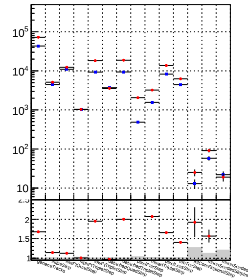
Number —●— DQM_BDT_mkFit_time
