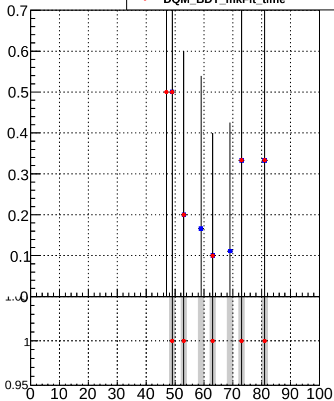
■ DQM_mkFit_time ● DQM_BDT_mkFit_time
