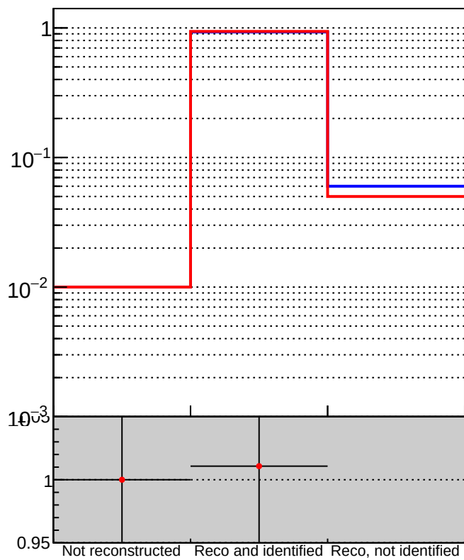
TruePVLocationIndexInRecoVertexCollectionCumulative
