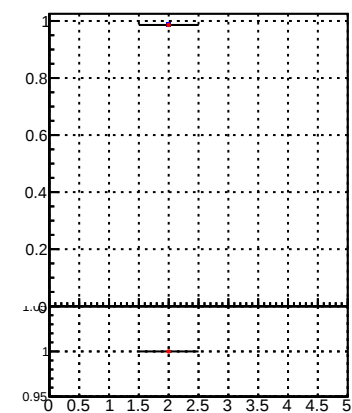
Fake rate vs hit Legend: DQM_mkFit_time (grey shaded region), DQM_BDT_mkFit_time (red dot with error bars)
