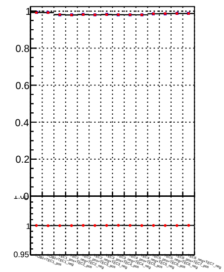
Fake rate vs. — DQM_mkFit_time — DQM_BDT_mkFit_time
