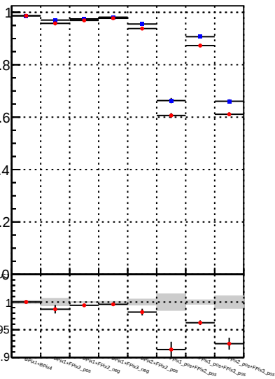
Fake rate vs. DQM_mkFit_time DQM_BDT_mkFit_time
