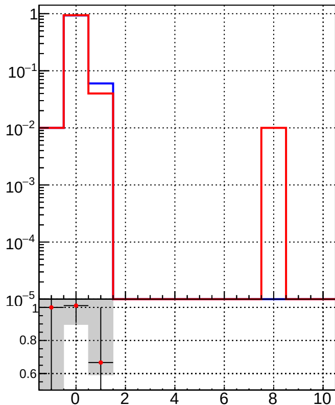
TruePVLocationIndexInRecoVertexCollection
