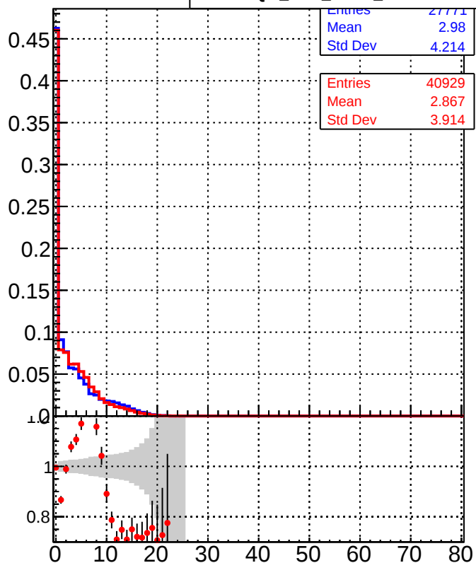
Legend: DQM_mkFit_time (Blue line with squares) DQM_BDT_mkFit_time (Red line with circles)
