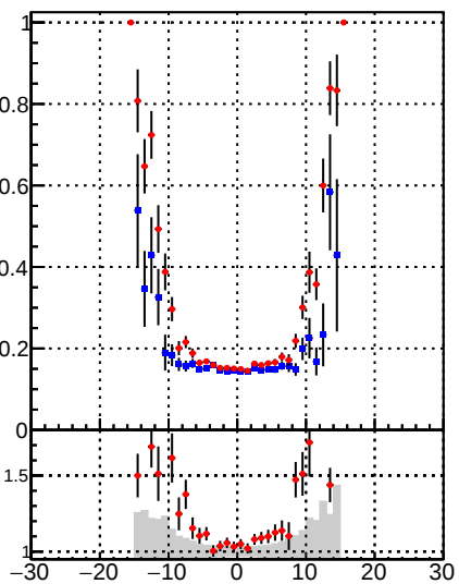
Fake rate vs d —●— DQM_mkFit_time —●— DQM_BDT_mkFit_time
