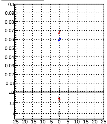
—●— DQM_mkFit_time —●— DQM_BDT_mkFit_time
