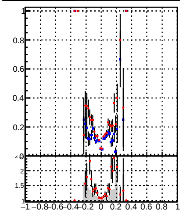
—●— DQM_mkFit_time —●— DQM_BDT_mkFit_time
