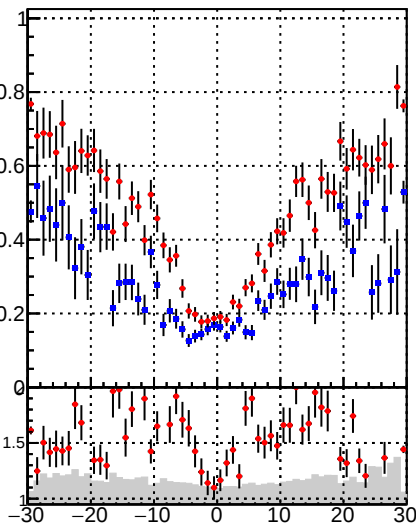
—●— DQM_mkFit_time —●— DQM_BDT_mkFit_time
