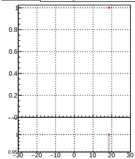
Fake rate vs \eta DQM_mkFit_time DQM_BDT_mkFit_time
